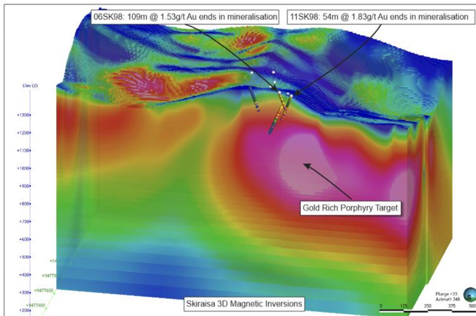
Figure 5: 3D magnetic model of the subsurface at Skiraisa highlights a highly magnetic target that represents a possible mineralized intrusive target.
