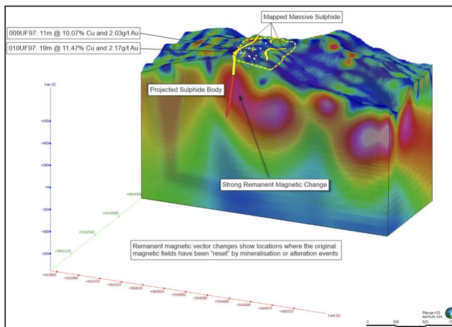
Figure 3: 3D magnetic model of the subsurface at Ufuo highlights a highly magnetic target that represents a possible mineralized intrusive target.
