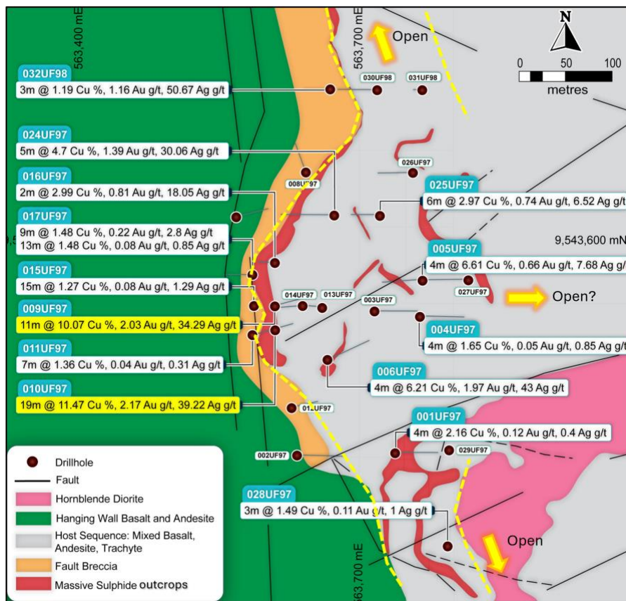
Figure 2: One of five prospects within the Ufuo Polymetallic Massive Sulfide District.
