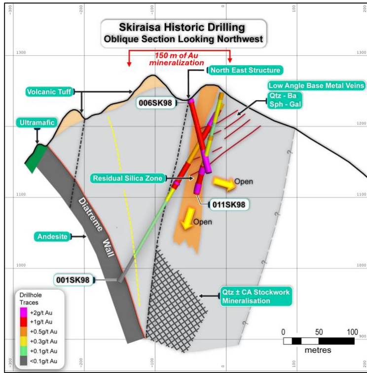
Figure 4: Cross section of the Skiraisa gold diatreme breccia, showing historical drilling and mineralization open to depth and to the east.
