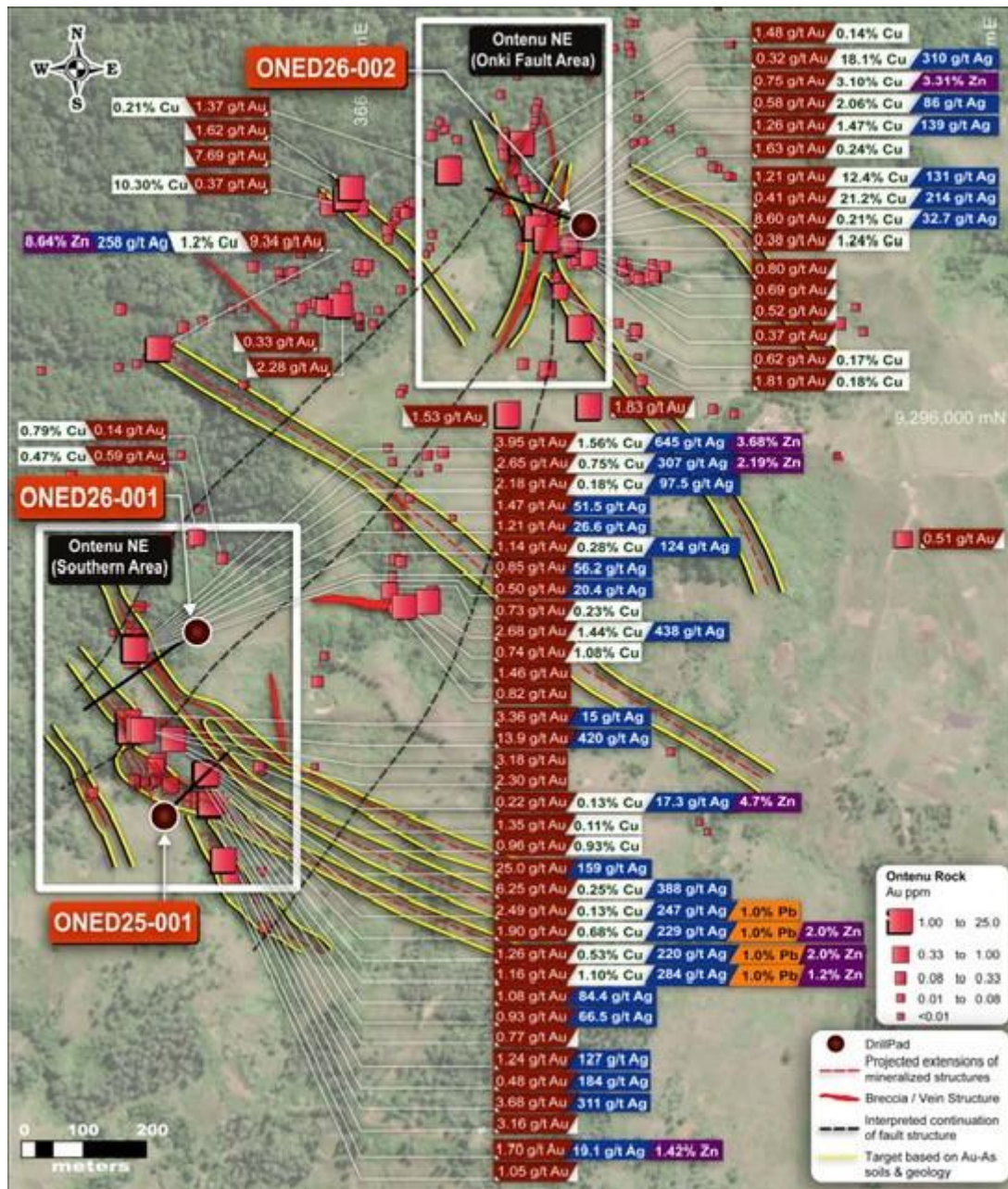
Figure 5 Ontenu NE target area with rock samples and soil anomalies
