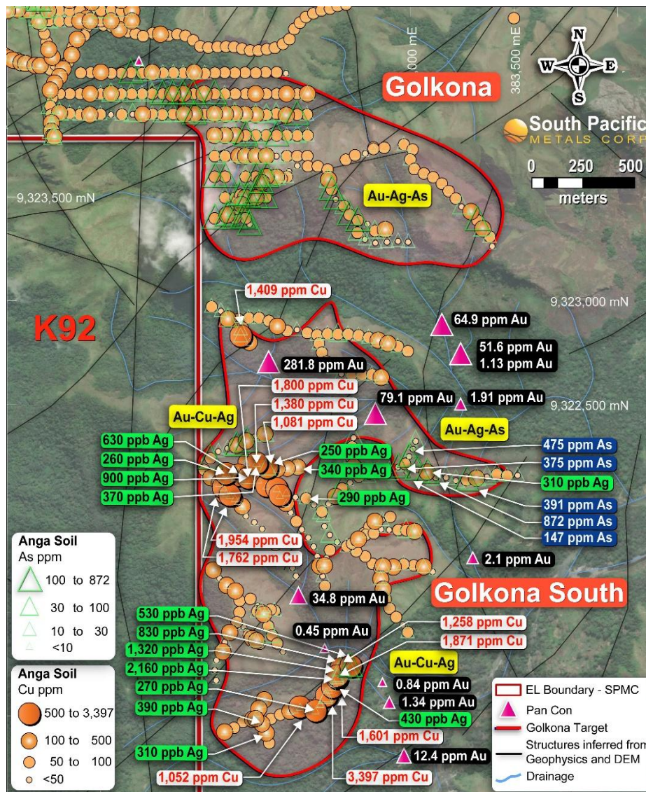
Figure 12 Cu-Ag-As in soils at Golkona and Golkona South
